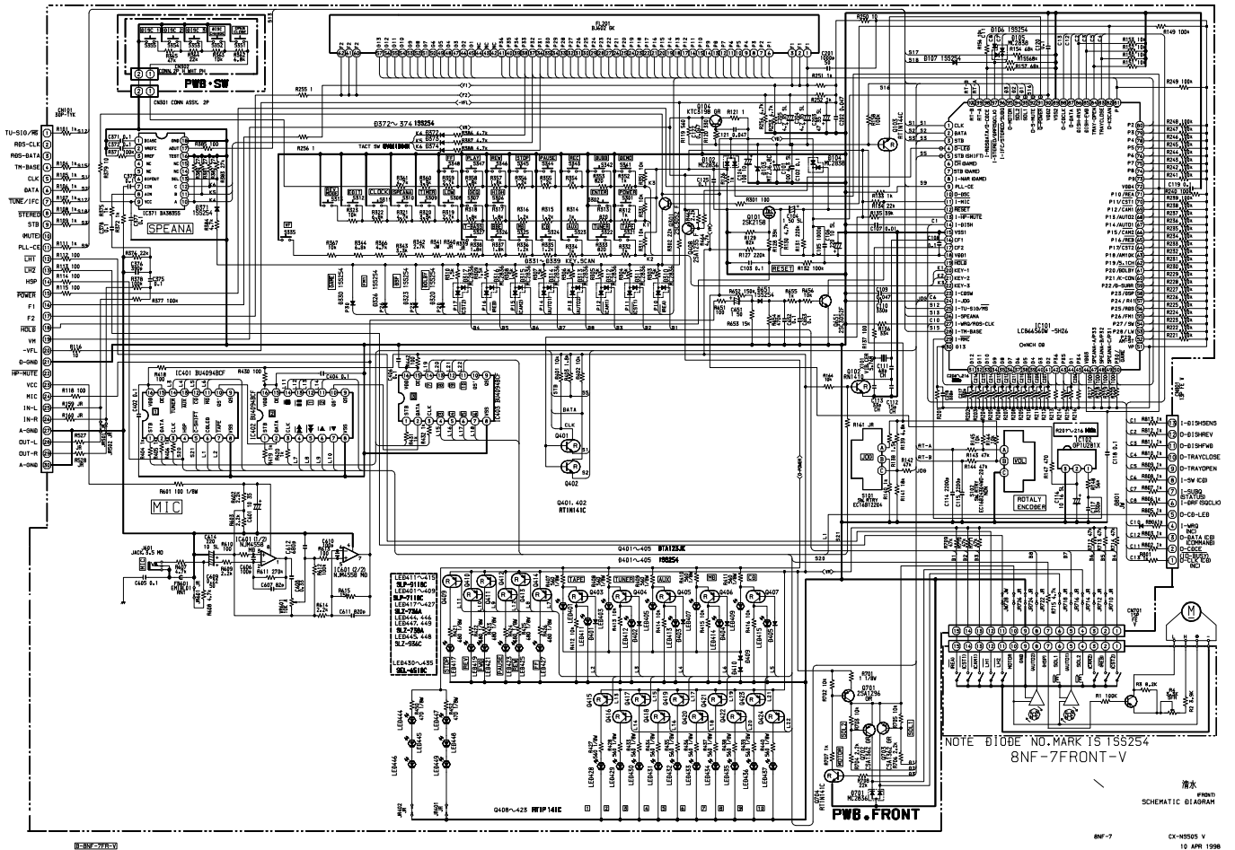
SCHEMATIC DIAGRAM - 5 (505V : FRONT)
