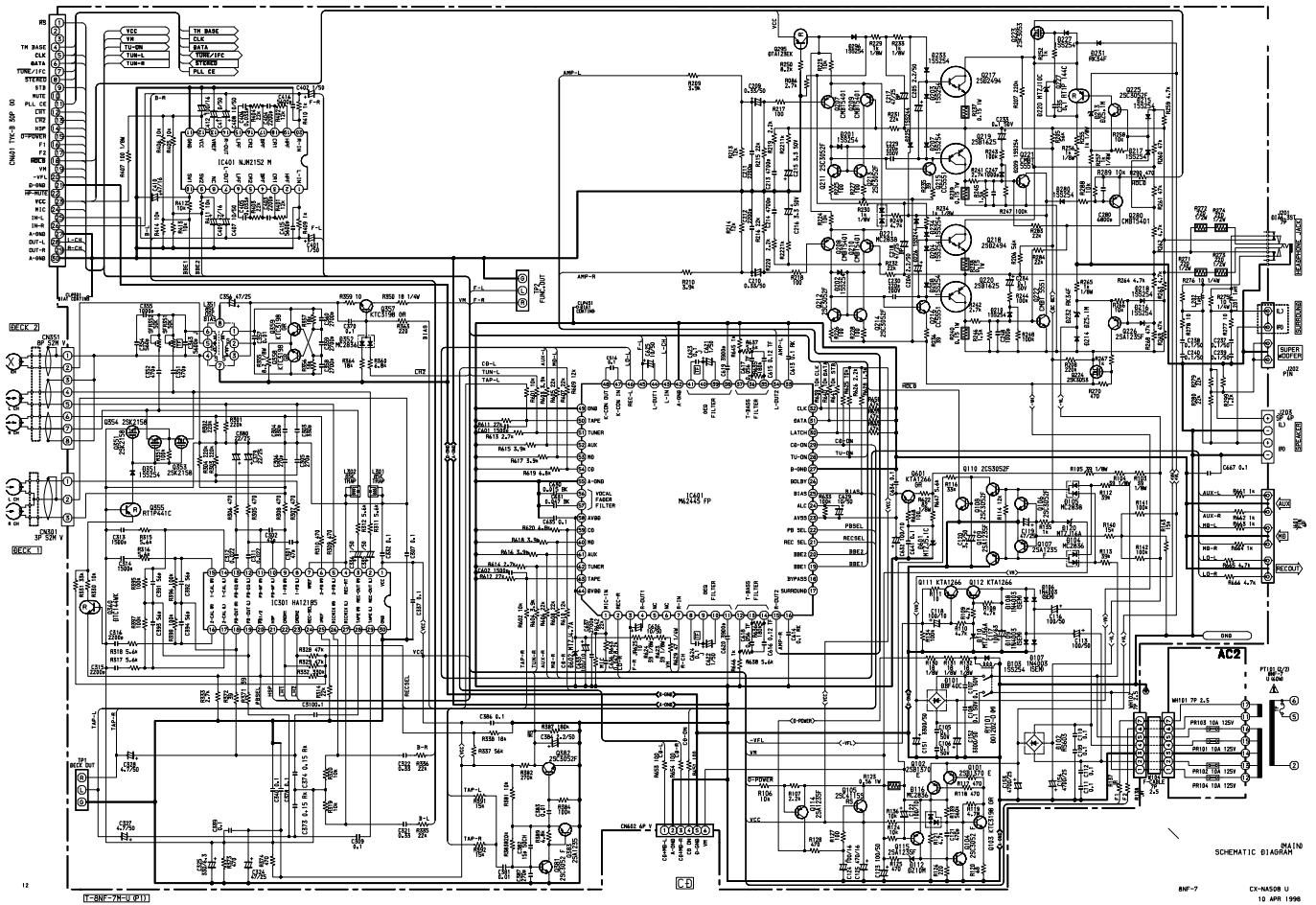
SCHEMATIC DIAGRAM - 2 (508U : MAIN)
