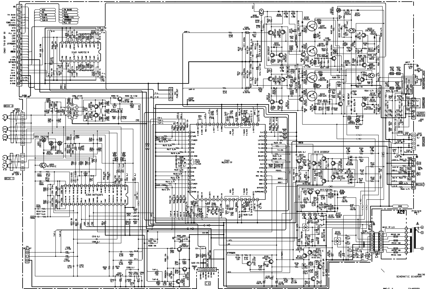
SCHEMATIC DIAGRAM - 1 (505V : MAIN)
